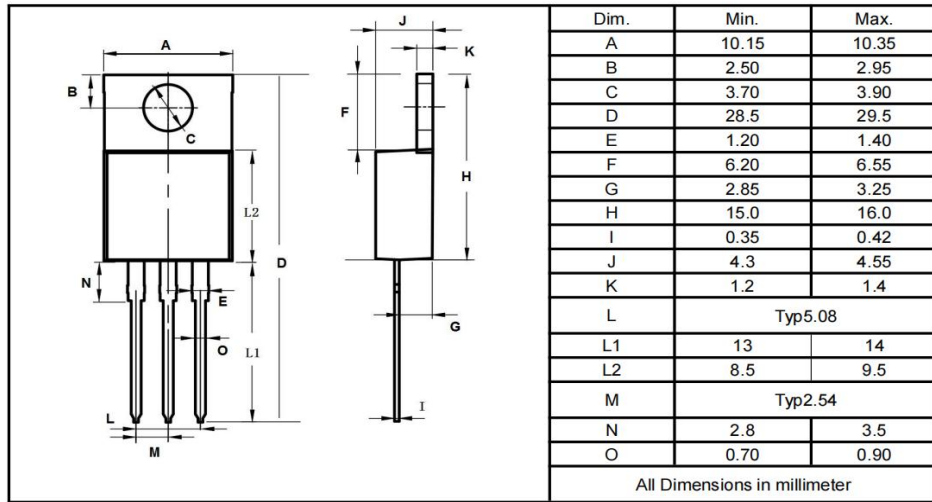
TO-220AB
